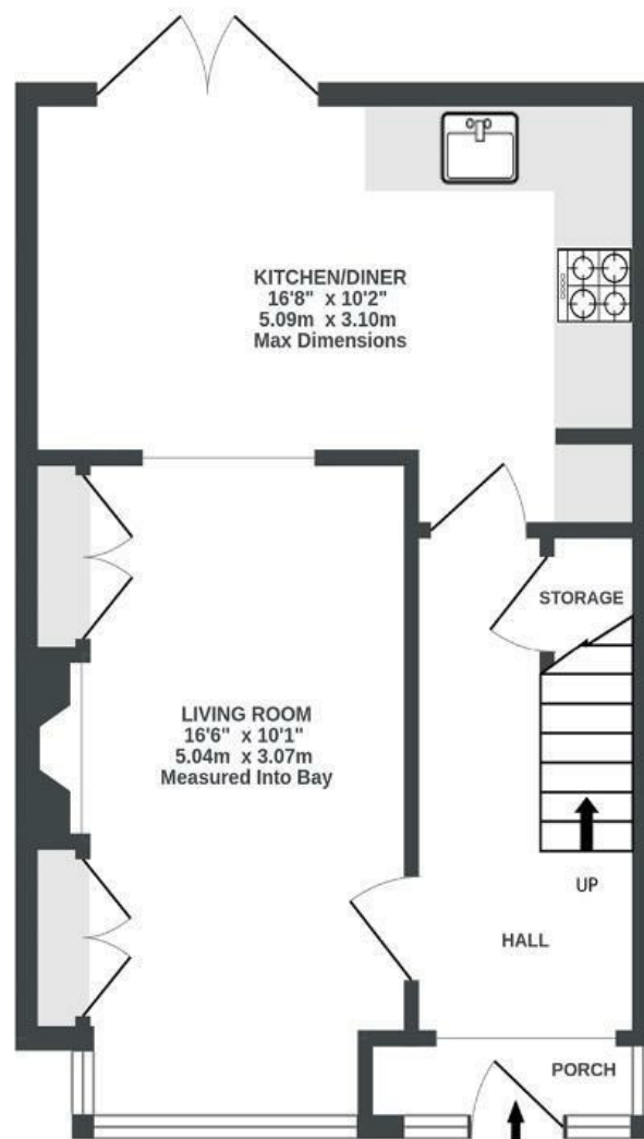
GROUND FLOOR 393 sq.ft. (36.5 sq.m.) approx.
